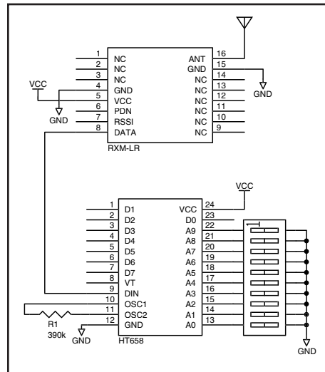
Figure 6: LR Receiver and HT658 Schematic
